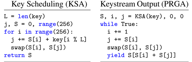
Figure 4: Implementation of RC4 in Python-like pseudocode. All additions are carried out modulo 256.
